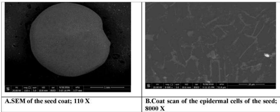
Figure 2. Seed Morphology and Coat Scan of Lotus ornithopodioides L. A.SEM of the seed coat; 110 X. B.Coat scan of the epidermal cells of the seed; 8000 X. Tribe 1. Loteae or Coronilleae, Genus: Tetragonolobus , Tetragonolobus purpureus Moench. Seed length: 2.5–4 mm. Width: 2–3.3 mm. Coat: glabrous. Texture: dull. Using a coat scan electron microscope at coat scan of the seed epidermal cells, power zoom 59 X (Figure 3A) & 8000X (Figure 3B), showed the following: raised and depressed anticlinal walls, holed outer periclinal wall, rugose and punctuate coat scan patterns, and glabrous anticlinal wall texture with bigger cells 2.196–2.914 µm wide.
